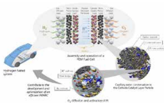
固体高分子形燃料電池内のマイクロ・ナノスケール熱流動解析 Micro- and nanoscale analysis of thermo-fluid transport in proton exchange membrane fuel cells
