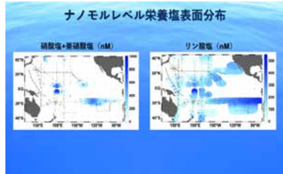
高感度分析で得られた太平洋表層におけるナノモルレベル栄養塩分布 Surface distribution of nanomolar nutrients across the oligotrophic Pacific Ocean revealed by highly sensitive analyses
