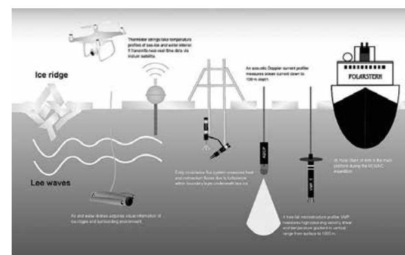
砕氷船を用いた北極海での海氷・海洋観測の模式図 Illustration of ice/ocean observation in the Arctic Ocean, with an ice breaker
